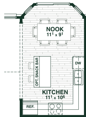
Optional Kitchen
